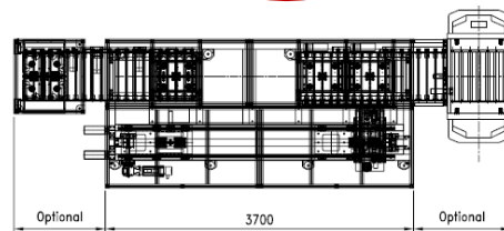
ASRS Robot
