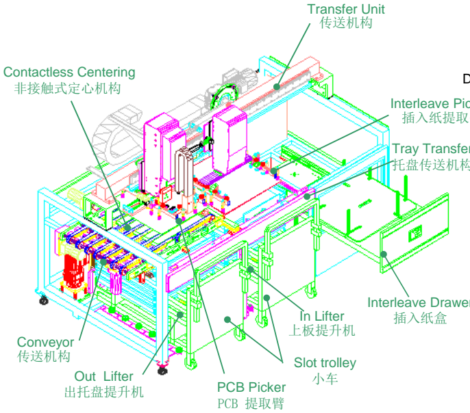
Tray Transfer 托盘传送机构
